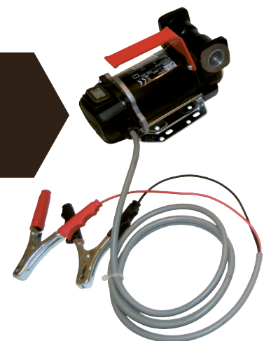
12/24v pumpar
